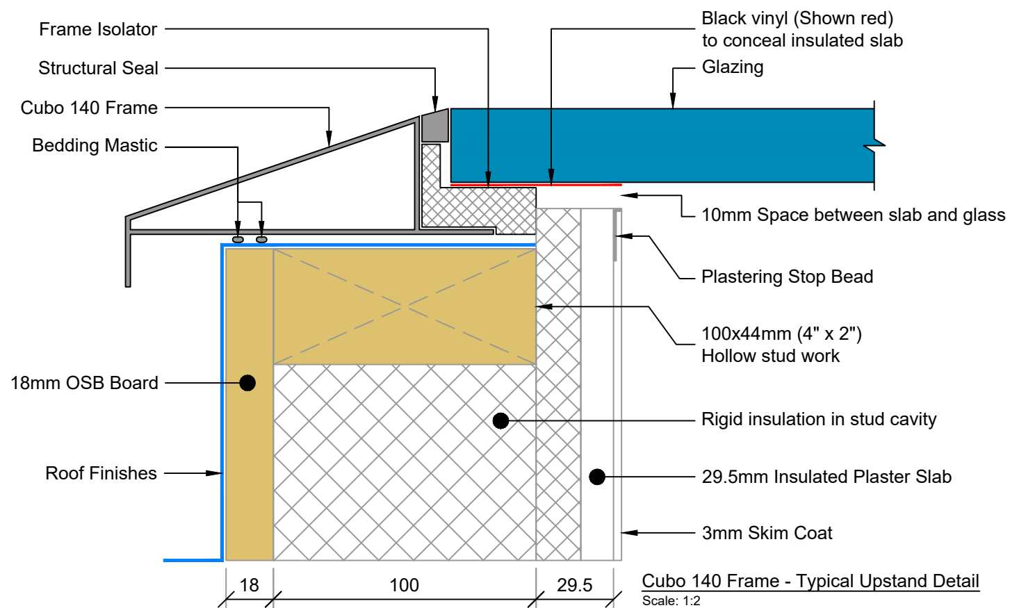
Cubo 140 Frame - Warm Roof Upstand Detail Scale: 1:2
